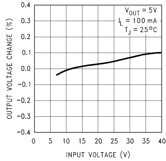
Line Regulation
