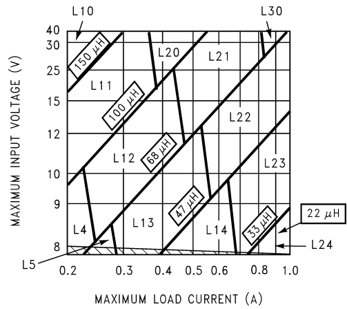
FIGURE 5. LM2672-5.0
