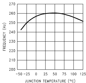
Switching Frequency
