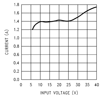
Peak Switch Current
