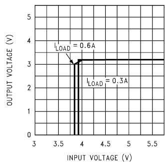
Dropout Voltage—3.3V Option
