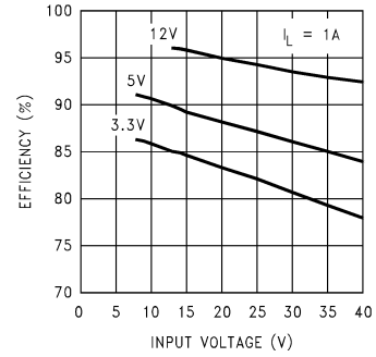
Efficiency
