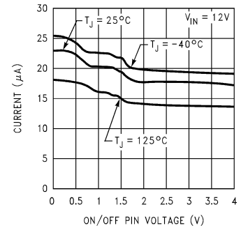
ON/OFF Pin Current (Sourcing)
